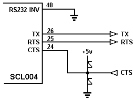
SIMPLE RS232 INTERFACE
