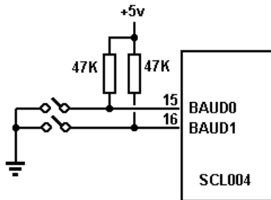
BAUD RATE CONNECTIONS
