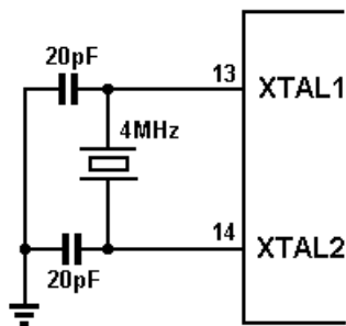
CLOCK CIRCUIT
