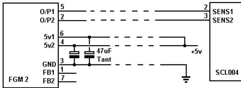
SENSOR CONNECTIONS
