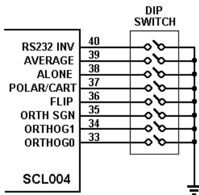
EXTERNAL CONTROL CONNECTIONS
