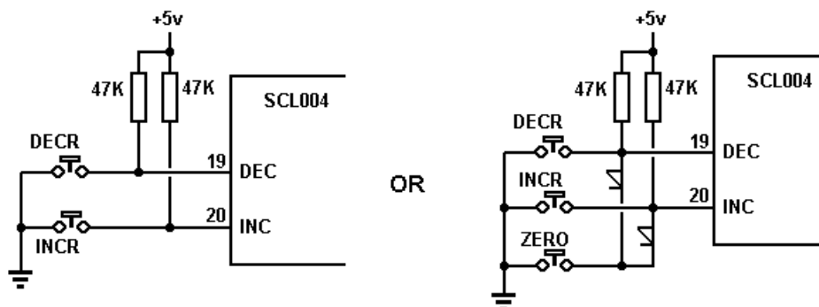
HEADING ADJUST CONNECTIONS
