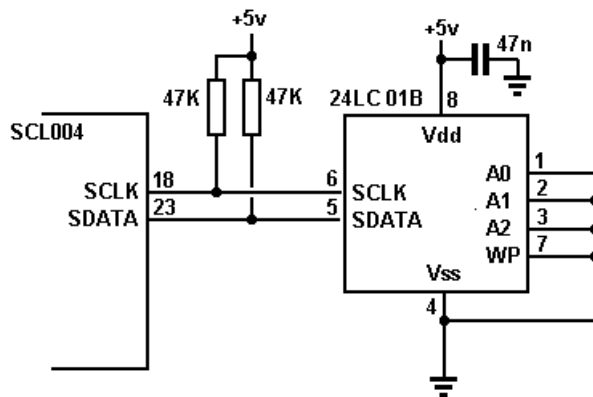
EEPROM CONNECTIONS
